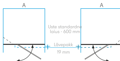
VASAKULE POOLE PAIGALDATAV UKS PEREMALE POOLE PAIGALDATAV UKS
